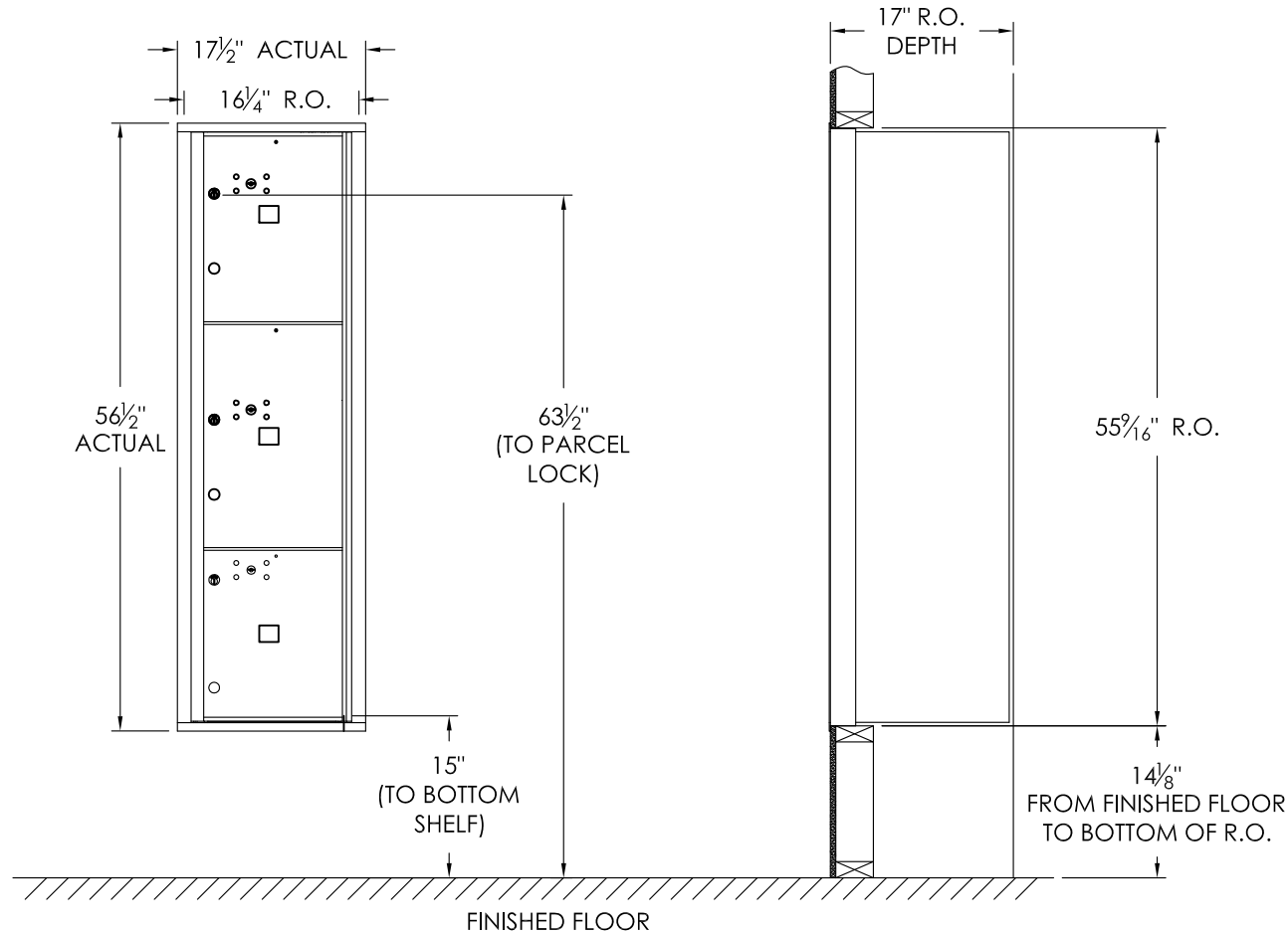
COMPARTMENT CHART
